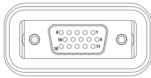
DB15 FEMALE
